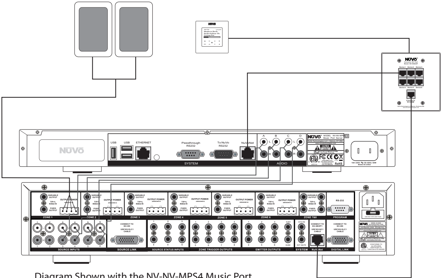
Diagram Shown with the NV-NV-MPS4 Music Port connected to the Grand Concerto System.
